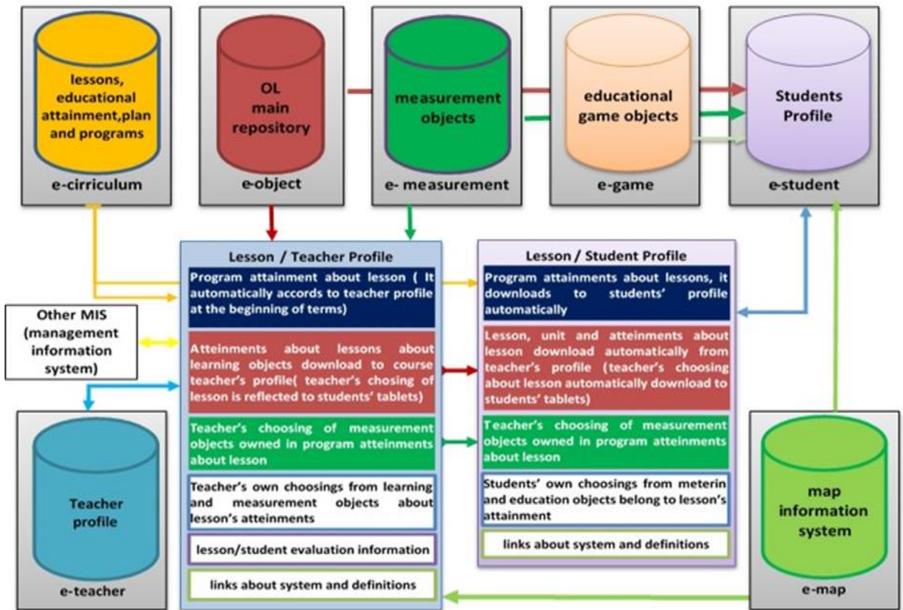
Figure 5: FATIH Project NLOMIS operation flow diagram
