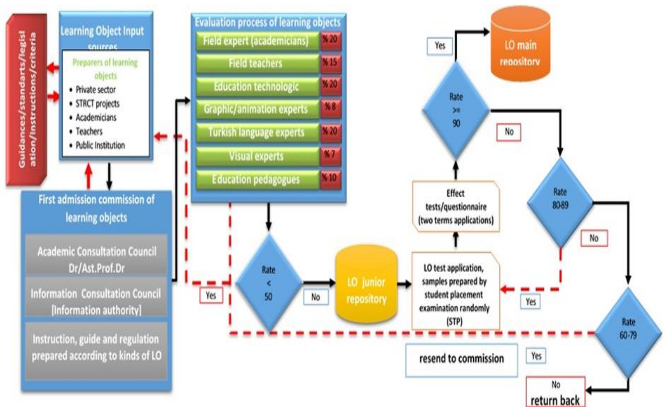
Figure 3: Structure and operation flow of NLOMIS
